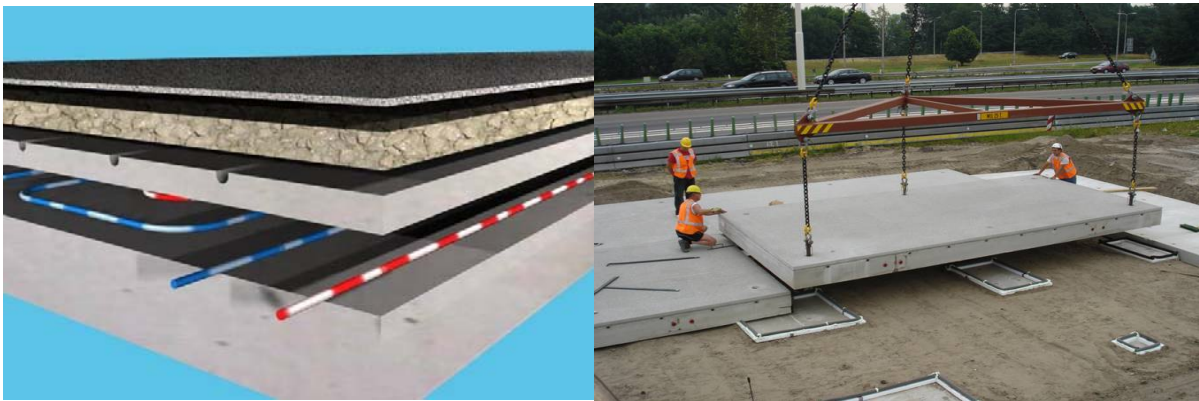
Figure 3. ModieSlab prefabricated concrete pavement.
